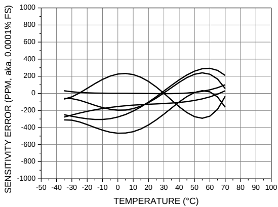
Figure 10a. Gyroscope Scale (Sensitivity) Error vs. Temperature
