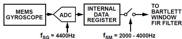
Figure 20. Gyroscope Data Sampling
