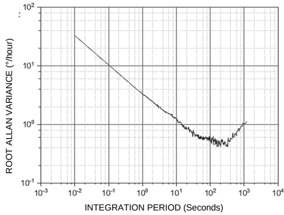
Figure 7. Gyroscope Allan Variance, 25°C
