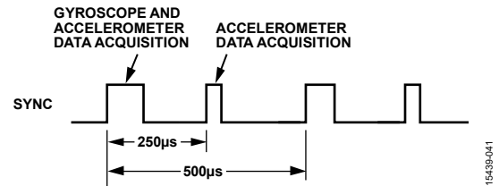
Figure 49. Sync Output Signal, Register MSC_CTRL, Bits[4:2] = 011
