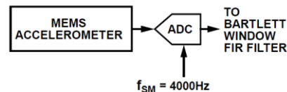
Figure 21. Accelerometer Data Sampling
