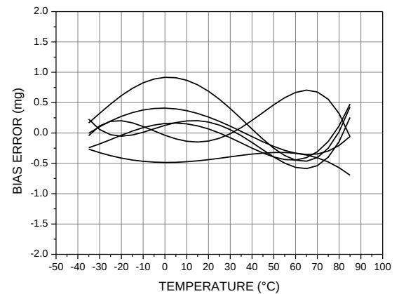
Figure 9b. Accelerometer Bias Error vs. Temperature
