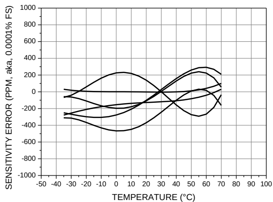
Figure 10a. Gyroscope Scale (Sensitivity) Error vs. Temperature
