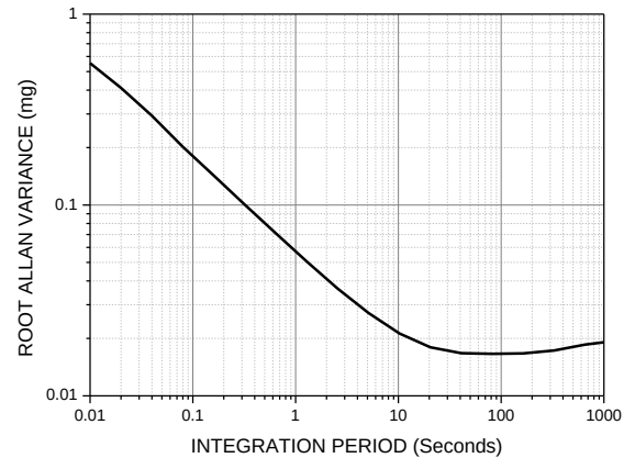
Figure 8. Accelerometer Allan Variance, 25°C
