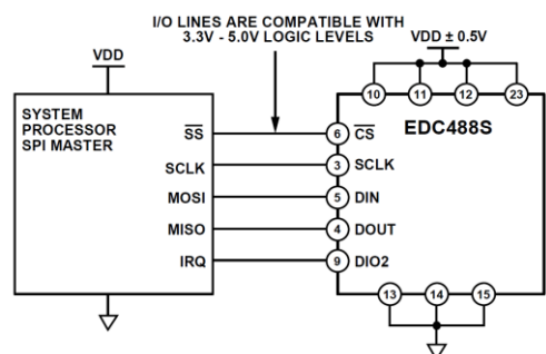
Figure 11. Electrical Connection Diagram
