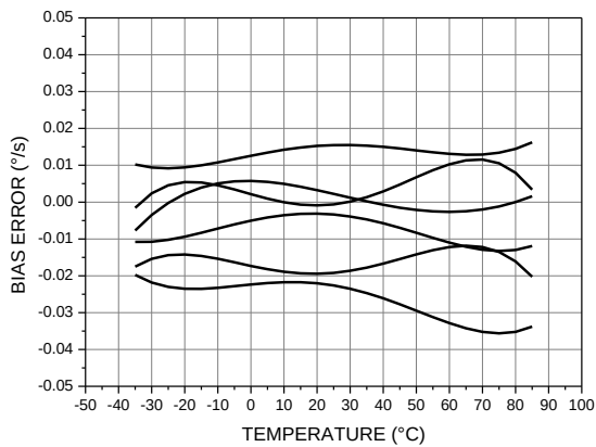
Figure 9a. Gyroscope Bias Error vs. Temperature
