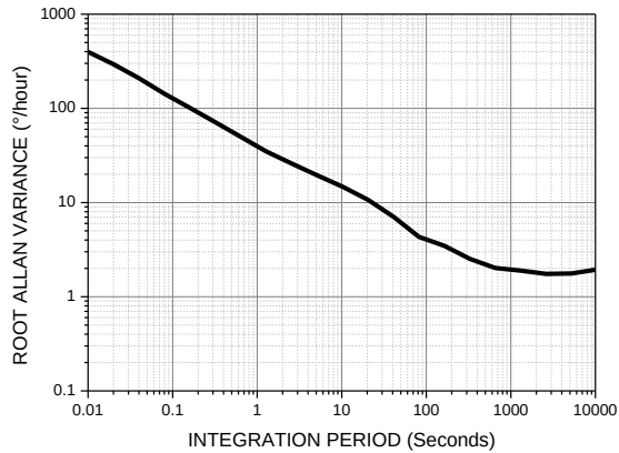
Figure 7. Gyroscope Allan Variance, 25°C
