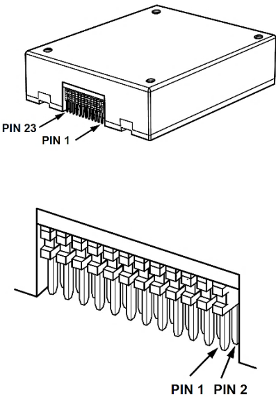
Figure 6. Axial Orientation (Top Side Facing Up)
