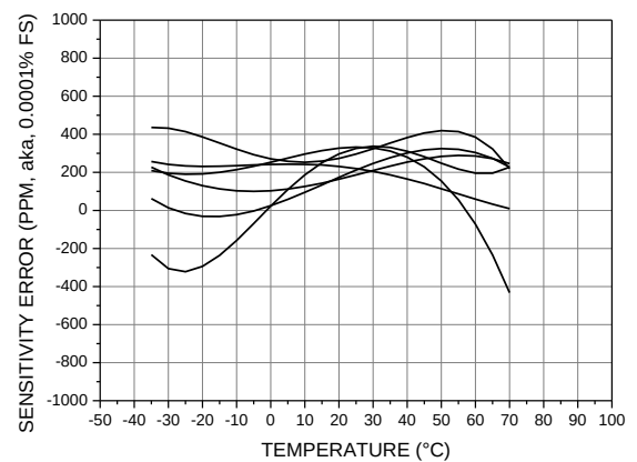
Figure 10b. Accelerometer Scale (Sensitivity) Error vs. Temperature
