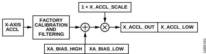
Figure 23. User Calibration Signal Path, Gyroscopes
